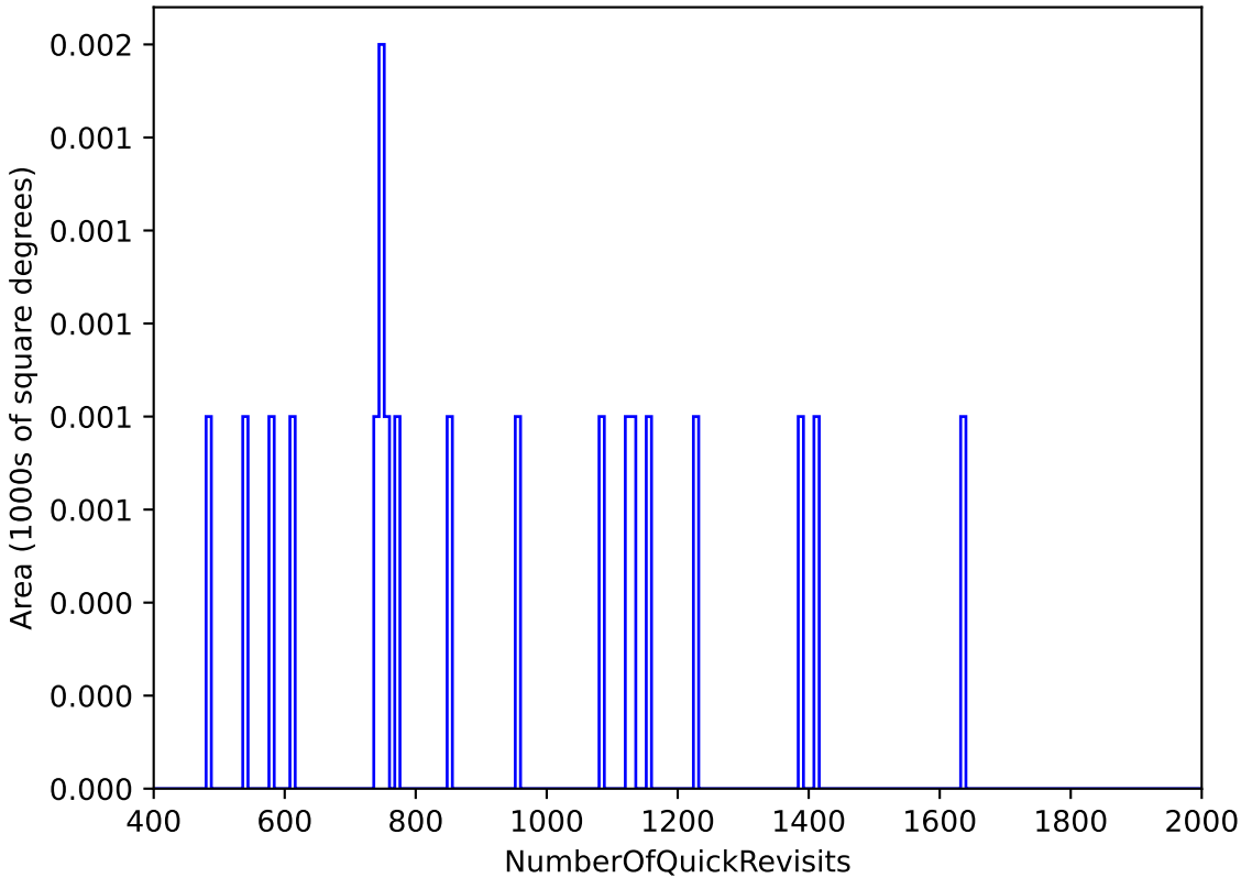
too_elab_r16_d3_ugrizy_v3.4_10yrs All sky: NumberOfQuickRevisits
