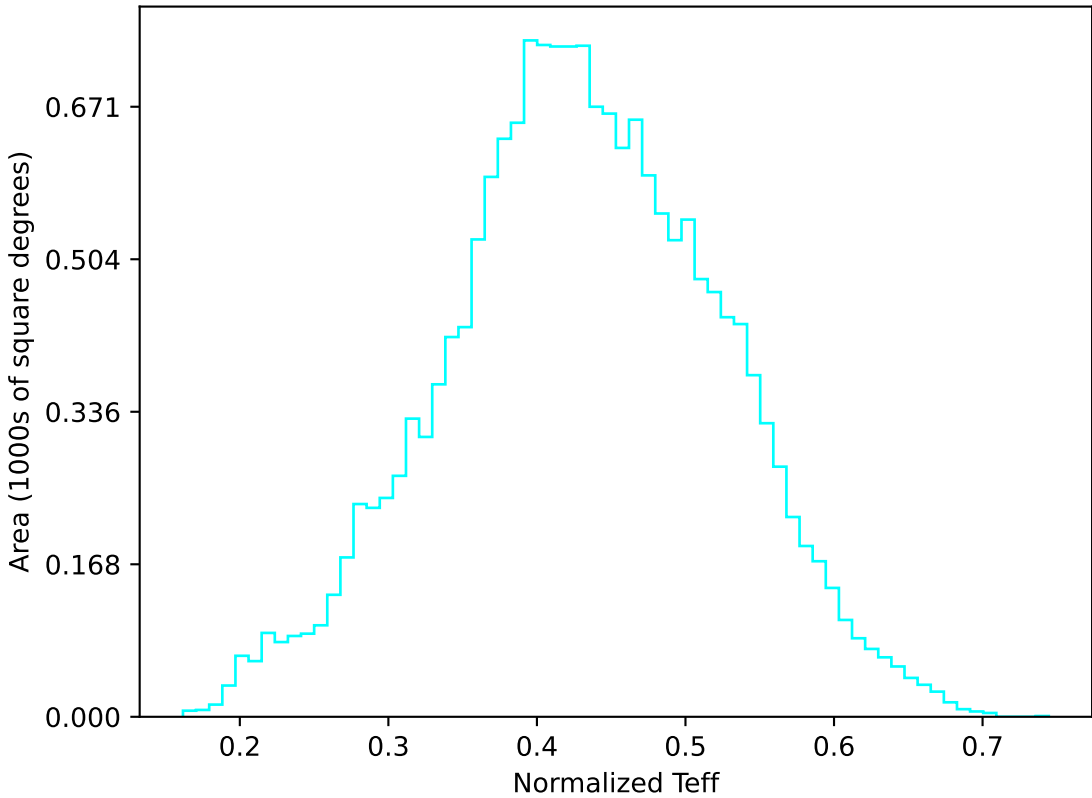
too_elab_r16_d3_ugrizy_v3.4_10yrs WFD u band: Normalized Teff
