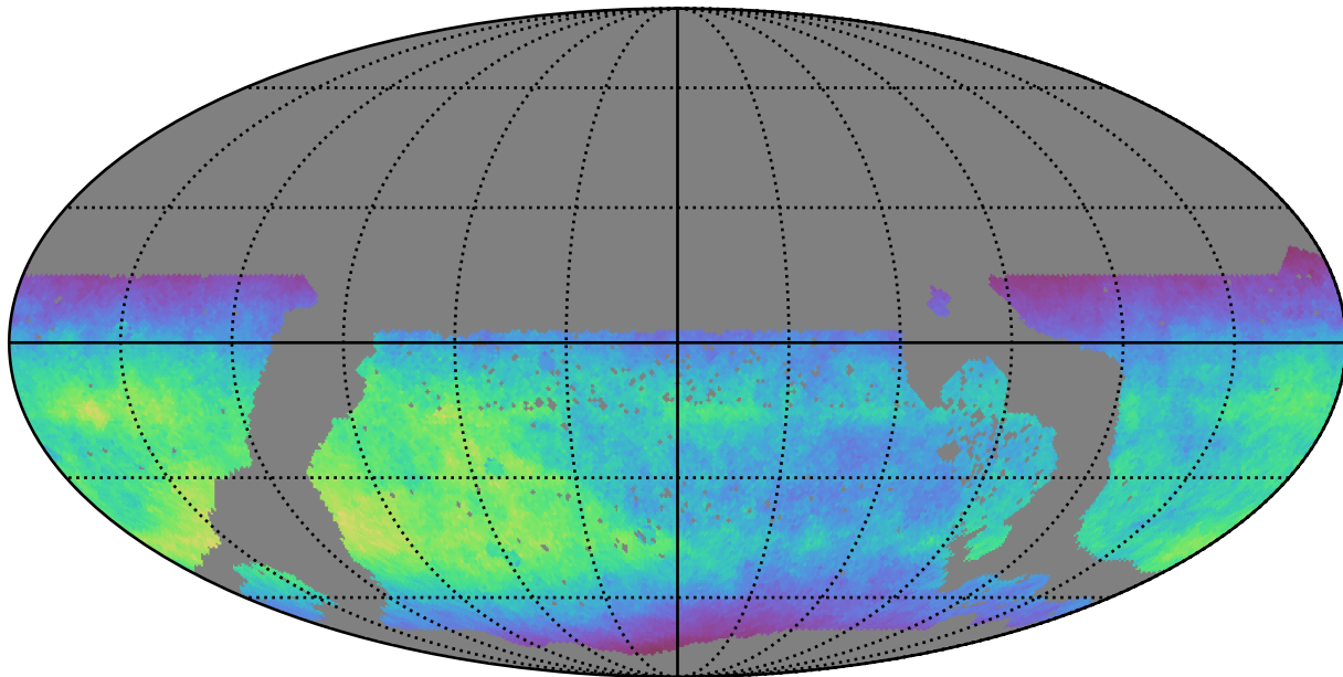
too_elab_r16_d3_ugrizy_v3.4_10yrs WFD i band: Normalized Teff
