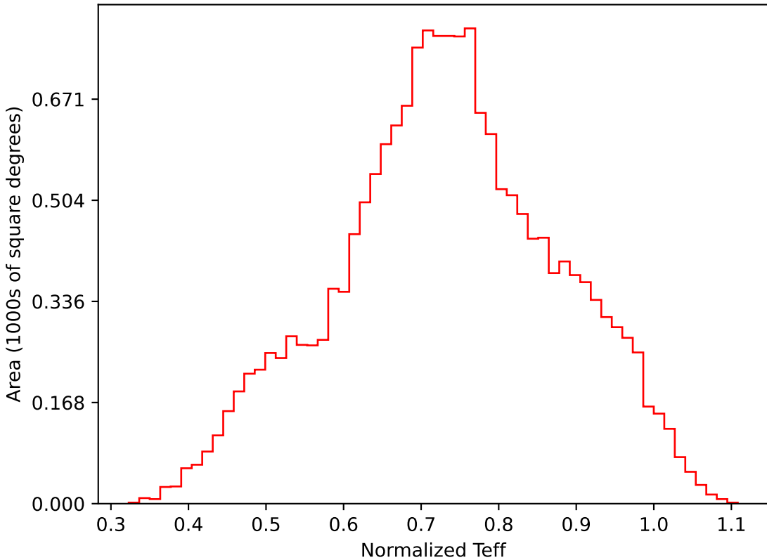
too_elab_r16_d3_ugrizy_v3.4_10yrs WFD i band: Normalized Teff
