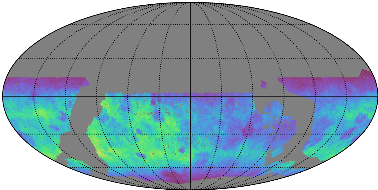
too_elab_r16_d3_ugrizy_v3.4_10yrs WFD g band: Normalized Teff
