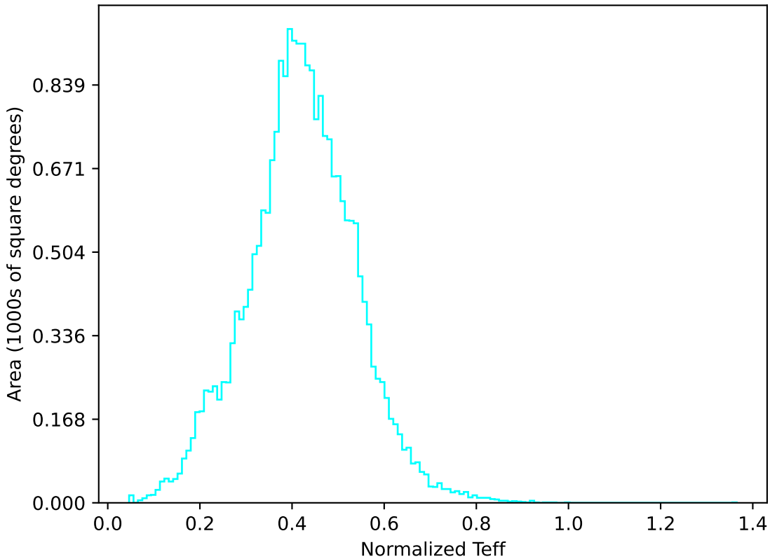
too_elab_r16_d3_ugrizy_v3.4_10yrs All sky u band: Normalized Teff
