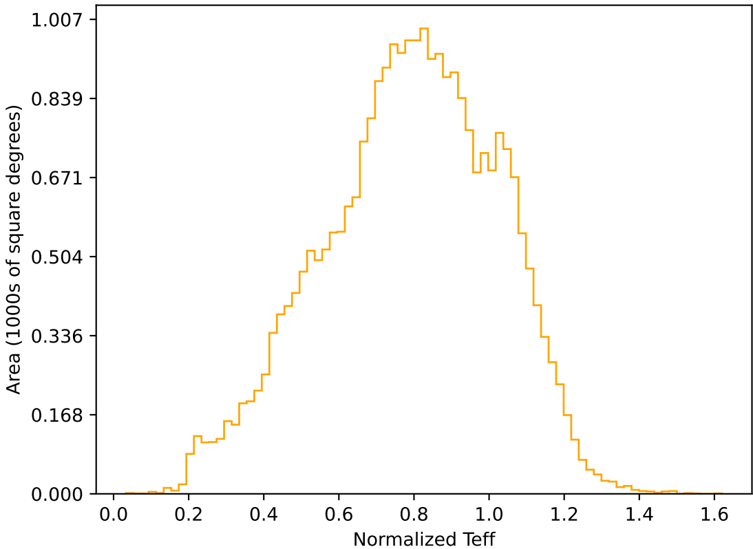
too_elab_r16_d3_ugrizy_v3.4_10yrs All sky r band: Normalized Teff
