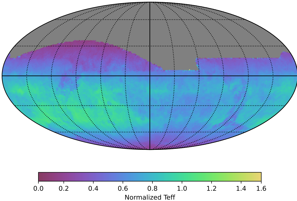
too_elab_r16_d3_ugrizy_v3.4_10yrs All sky i band: Normalized Teff
