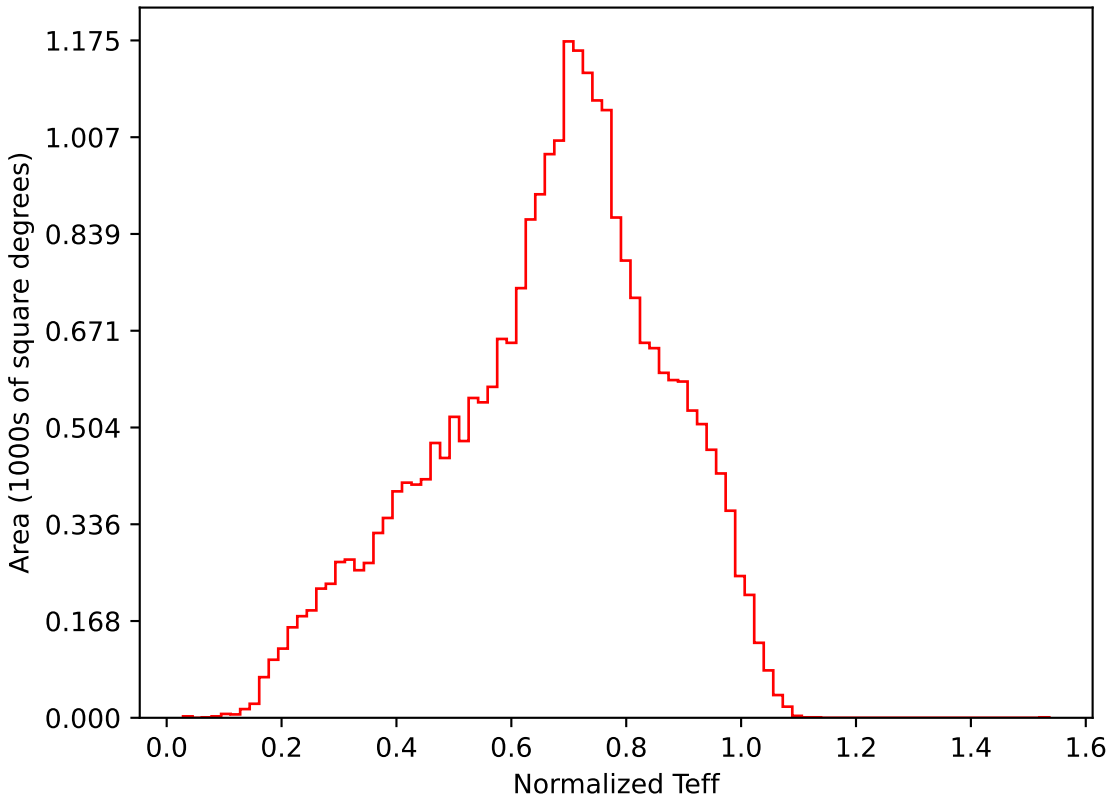
too_elab_r16_d3_ugrizy_v3.4_10yrs All sky i band: Normalized Teff
