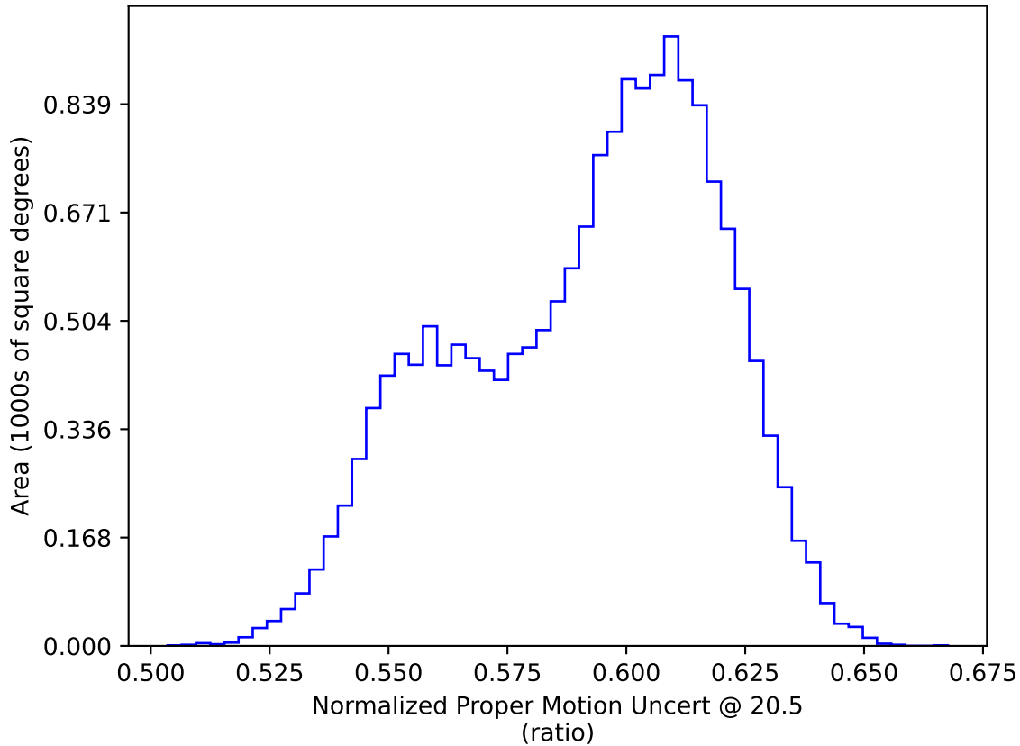
too_elab_r16_d3_ugrizy_v3.4_10yrs WFD: Normalized Proper Motion Uncert @ 20.5
