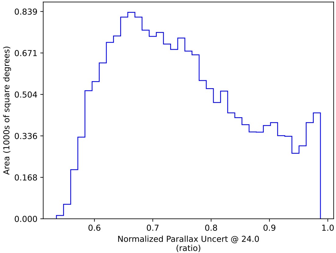
too_elab_r16_d3_ugrizy_v3.4_10yrs WFD: Normalized Parallax Uncert @ 24.0
