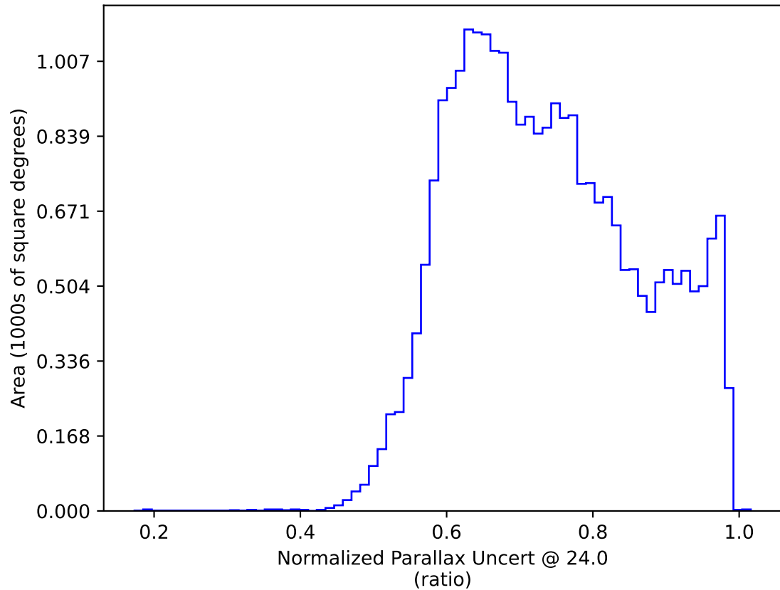
too_elab_r16_d3_ugrizy_v3.4_10yrs All sky: Normalized Parallax Uncert @ 24.0
