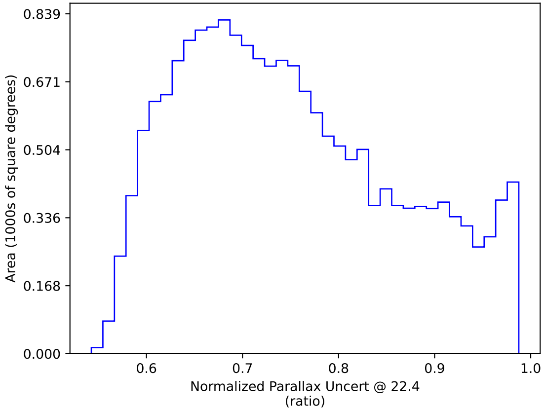
too_elab_r16_d3_ugrizy_v3.4_10yrs WFD: Normalized Parallax Uncert @ 22.4
