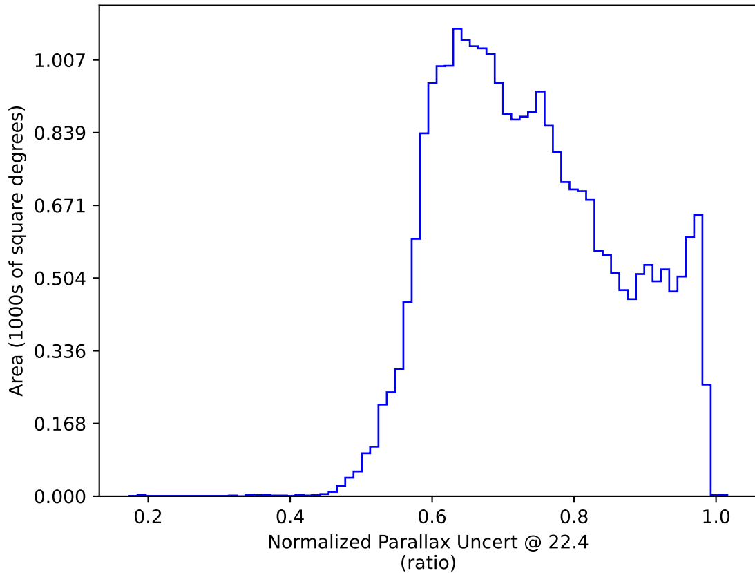
too_elab_r16_d3_ugrizy_v3.4_10yrs All sky: Normalized Parallax Uncert @ 22.4
