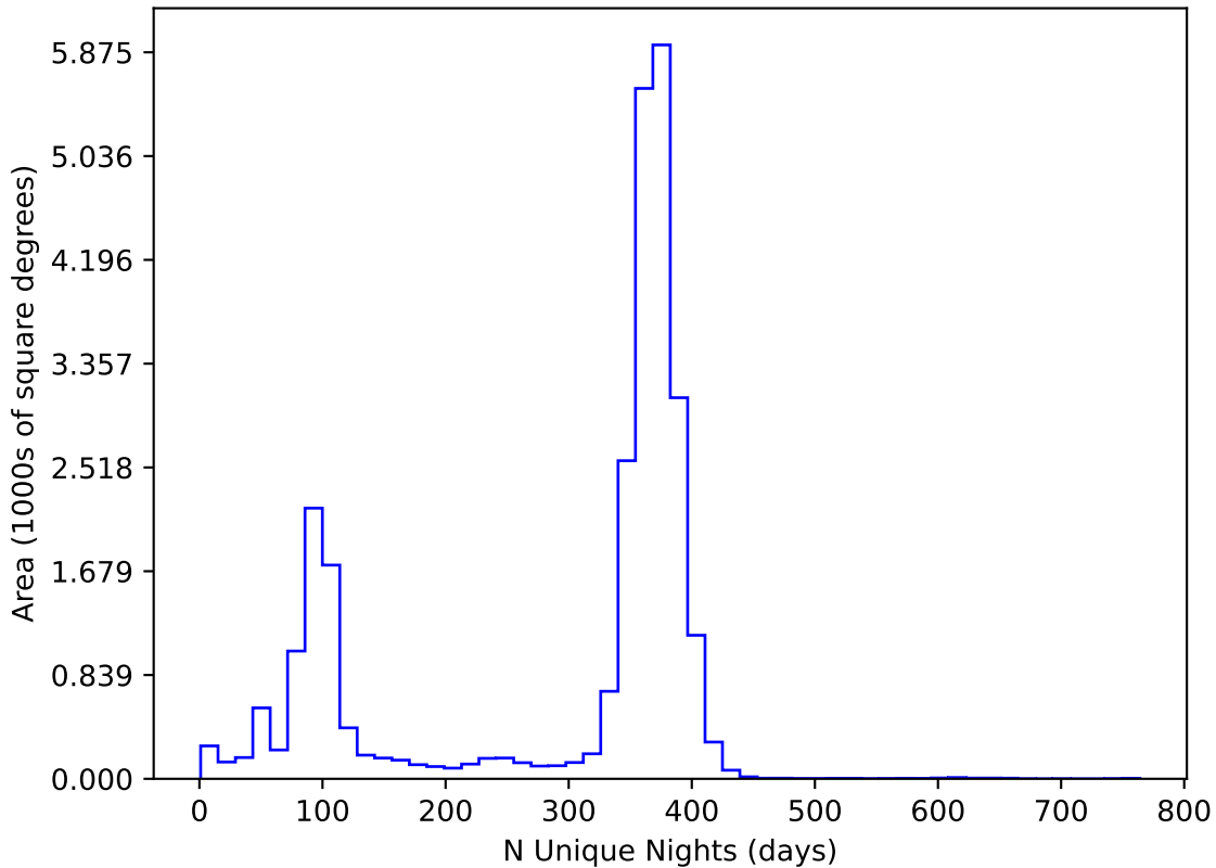
too_elab_r16_d3_ugrizy_v3.4_10yrs All sky all bands: N Unique Nights
