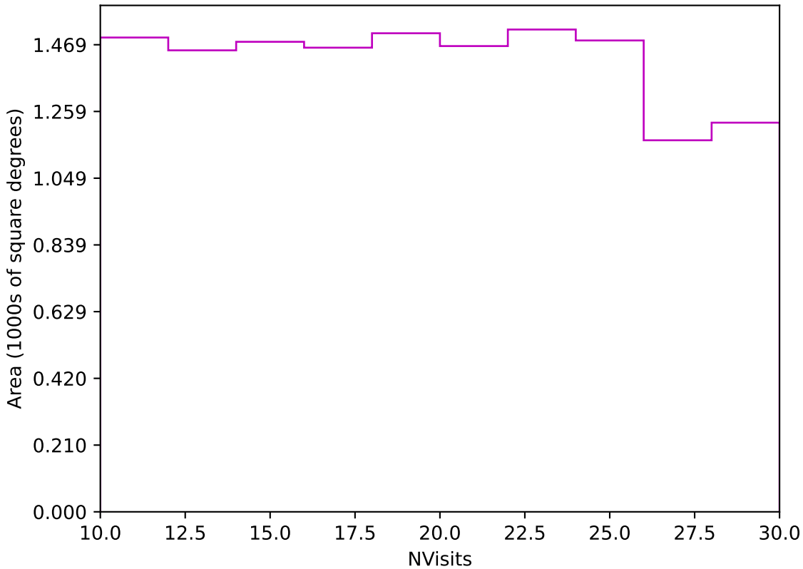
too_elab_r16_d3_ugrizy_v3.4_10yrs Yr 3-4 z band: NVisits
