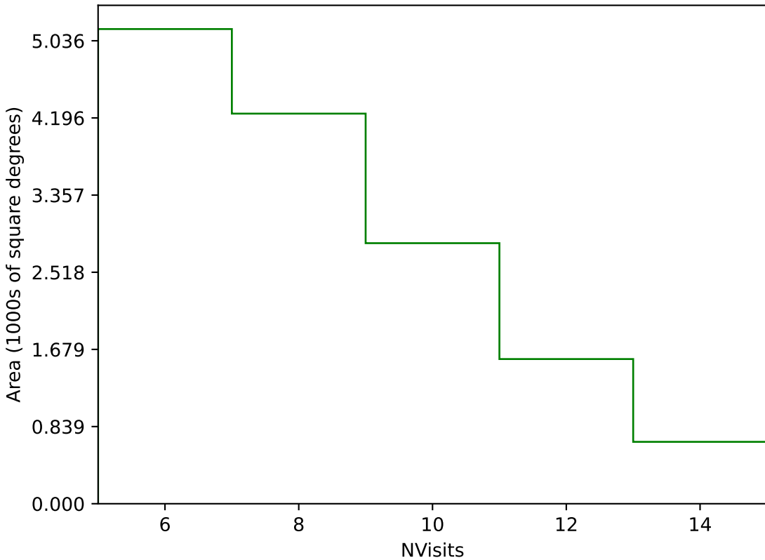
too_elab_r16_d3_ugrizy_v3.4_10yrs Yr 3-4 g band: NVisits
