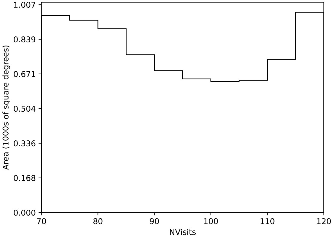
too_elab_r16_d3_ugrizy_v3.4_10yrs Yr 3-4 all bands: NVisits
