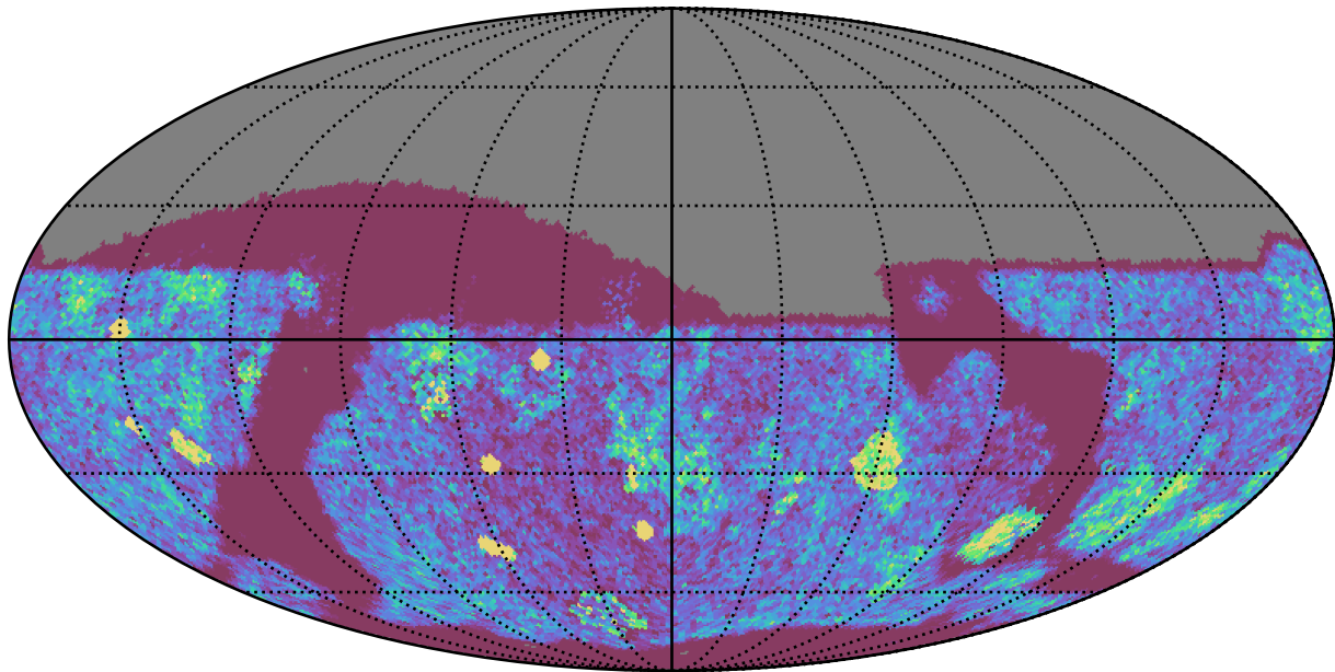
too_elab_r16_d3_ugrizy_v3.4_10yrs Yr 1 z band: NVisits
