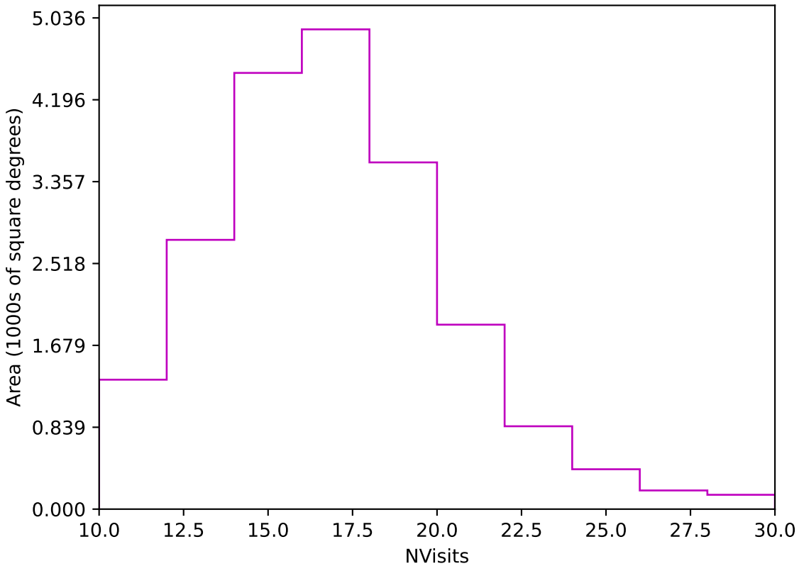
too_elab_r16_d3_ugrizy_v3.4_10yrs Yr 1 z band: NVisits
