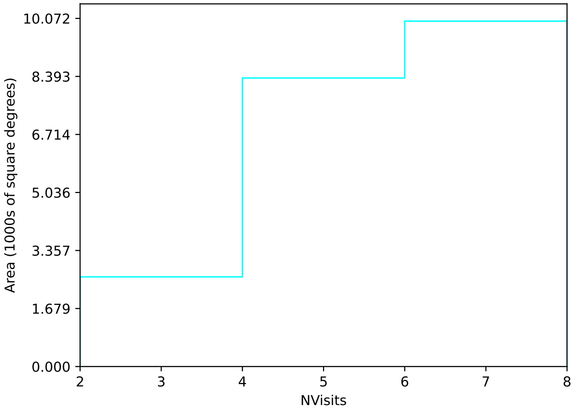
too_elab_r16_d3_ugrizy_v3.4_10yrs Yr 1 u band: NVisits
