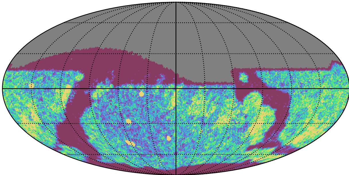
too_elab_r16_d3_ugrizy_v3.4_10yrs Yr 1 r band: NVisits
