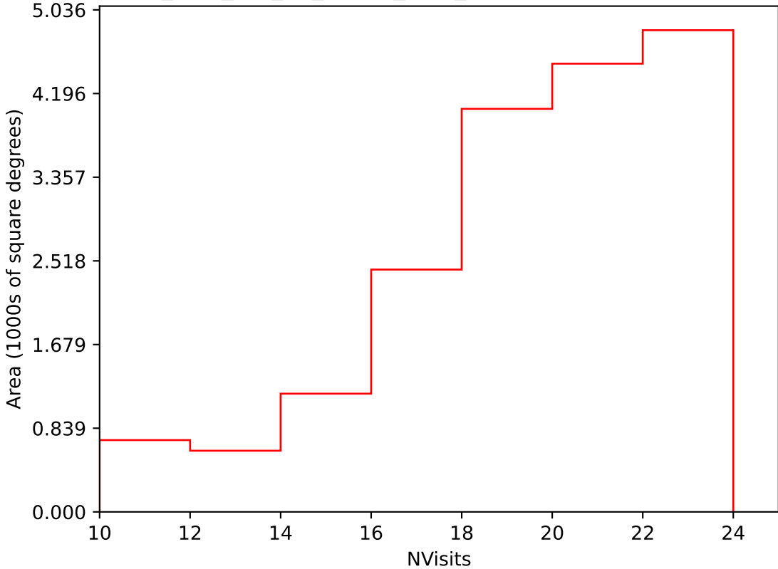
too_elab_r16_d3_ugrizy_v3.4_10yrs Yr 1 i band: NVisits
