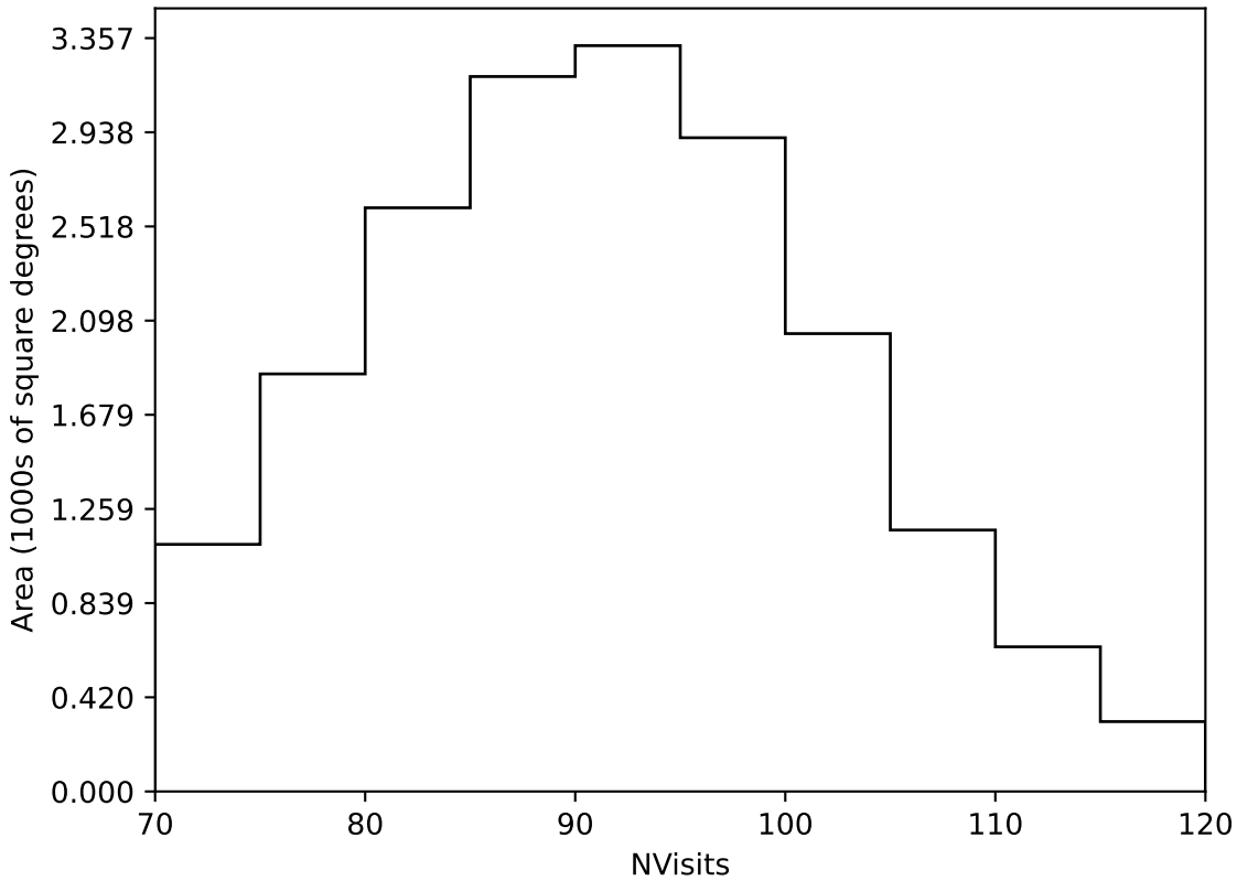
too_elab_r16_d3_ugrizy_v3.4_10yrs Yr 1 all bands: NVisits
