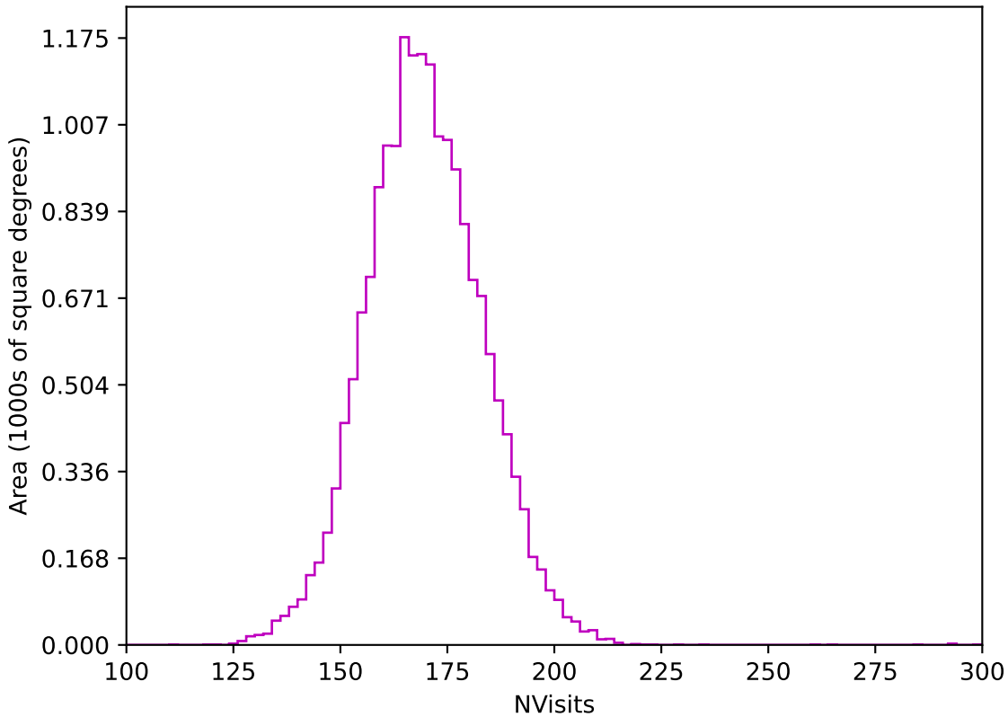
too_elab_r16_d3_ugrizy_v3.4_10yrs WFD z band: NVisits
