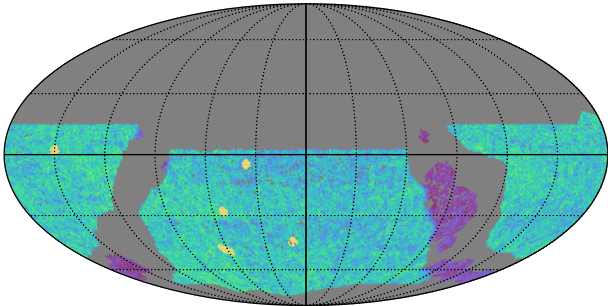
too_elab_r16_d3_ugrizy_v3.4_10yrs WFD u band: NVisits
