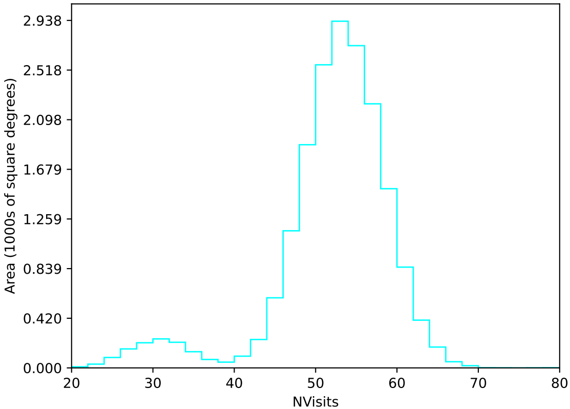
too_elab_r16_d3_ugrizy_v3.4_10yrs WFD u band: NVisits
