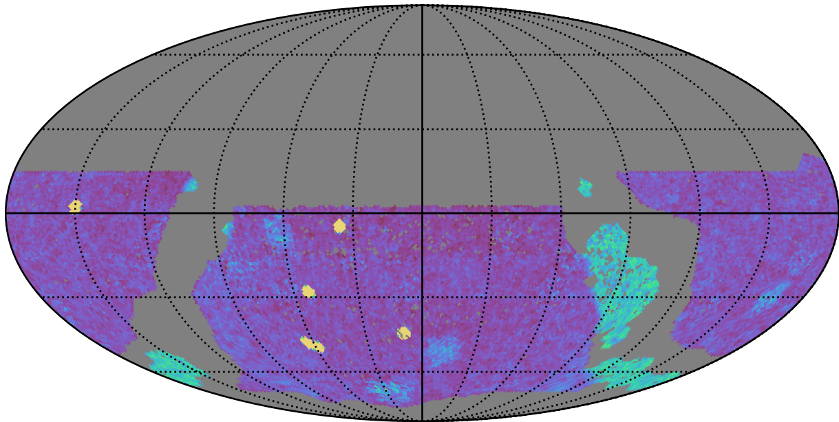
too_elab_r16_d3_ugrizy_v3.4_10yrs WFD g band: NVisits
