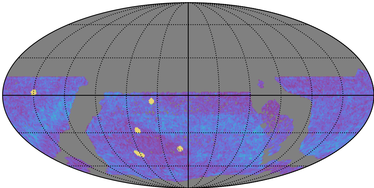
too_elab_r16_d3_ugrizy_v3.4_10yrs WFD all bands: NVisits
