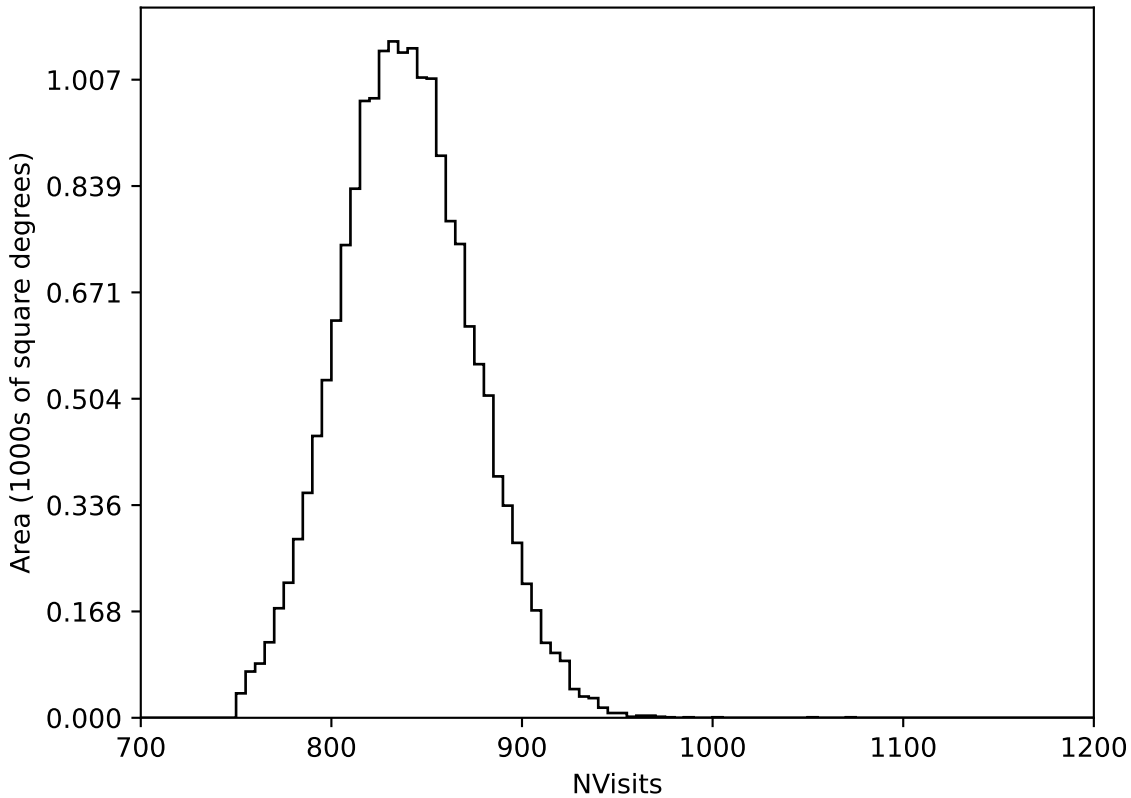
too_elab_r16_d3_ugrizy_v3.4_10yrs WFD all bands: NVisits
