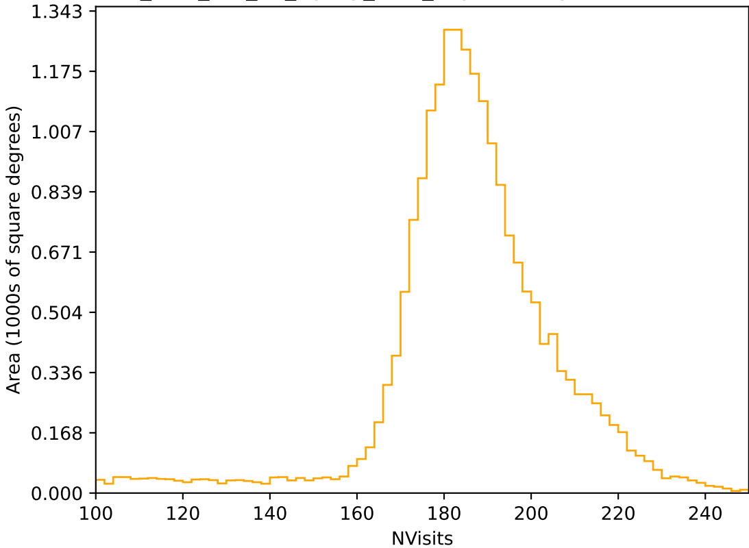
too_elab_r16_d3_ugrizy_v3.4_10yrs All sky r band: NVisits
