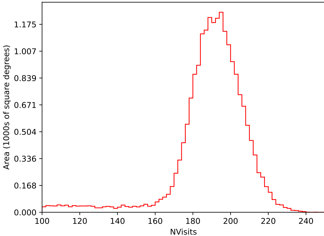
too_elab_r16_d3_ugrizy_v3.4_10yrs All sky i band: NVisits
