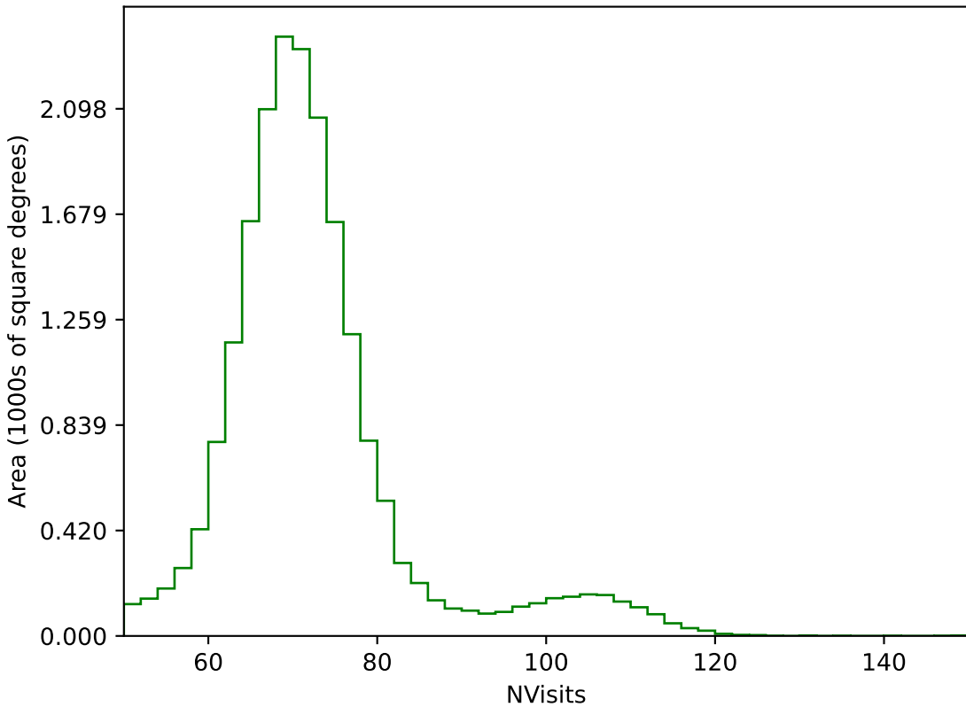
too_elab_r16_d3_ugrizy_v3.4_10yrs All sky g band: NVisits
