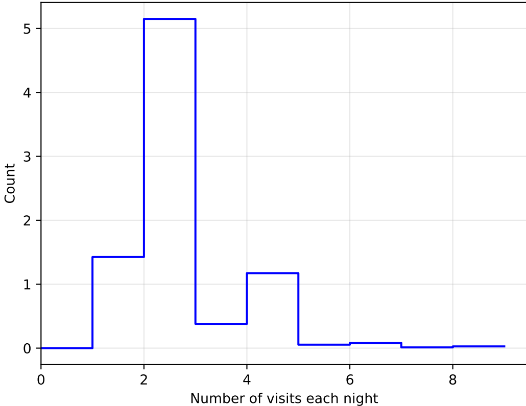
too_elab_r16_d3_ugrizy_v3.4_10yrs WFD: NVisitsPerNight 1e6
