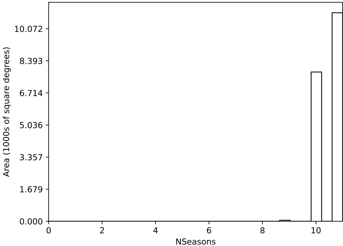
too_elab_r16_d3_ugrizy_v3.4_10yrs WFD all bands: NSeasons
