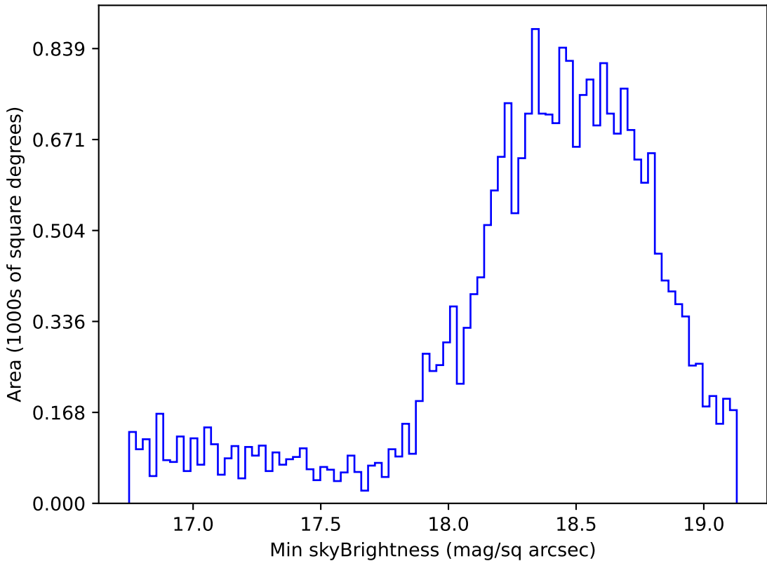
too_elab_r16_d3_ugrizy_v3.4_10yrs Yr 1 z band: Min skyBrightness
