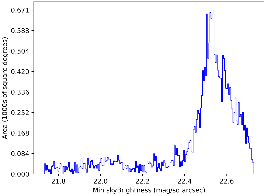
too_elab_r16_d3_ugrizy_v3.4_10yrs Yr 1 u band: Min skyBrightness
