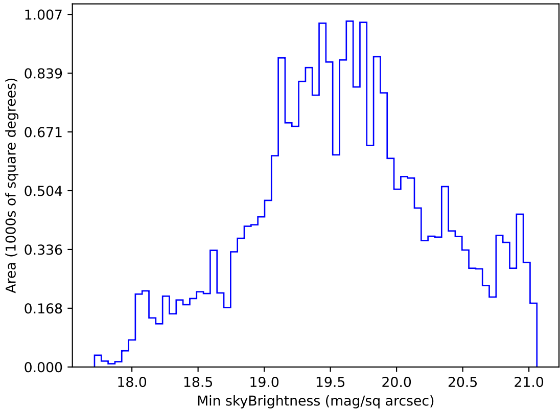
too_elab_r16_d3_ugrizy_v3.4_10yrs Yr 1 r band: Min skyBrightness
