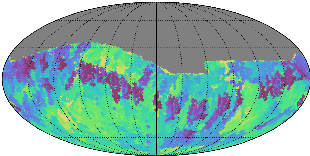
too_elab_r16_d3_ugrizy_v3.4_10yrs Yr 1 i band: Min skyBrightness
