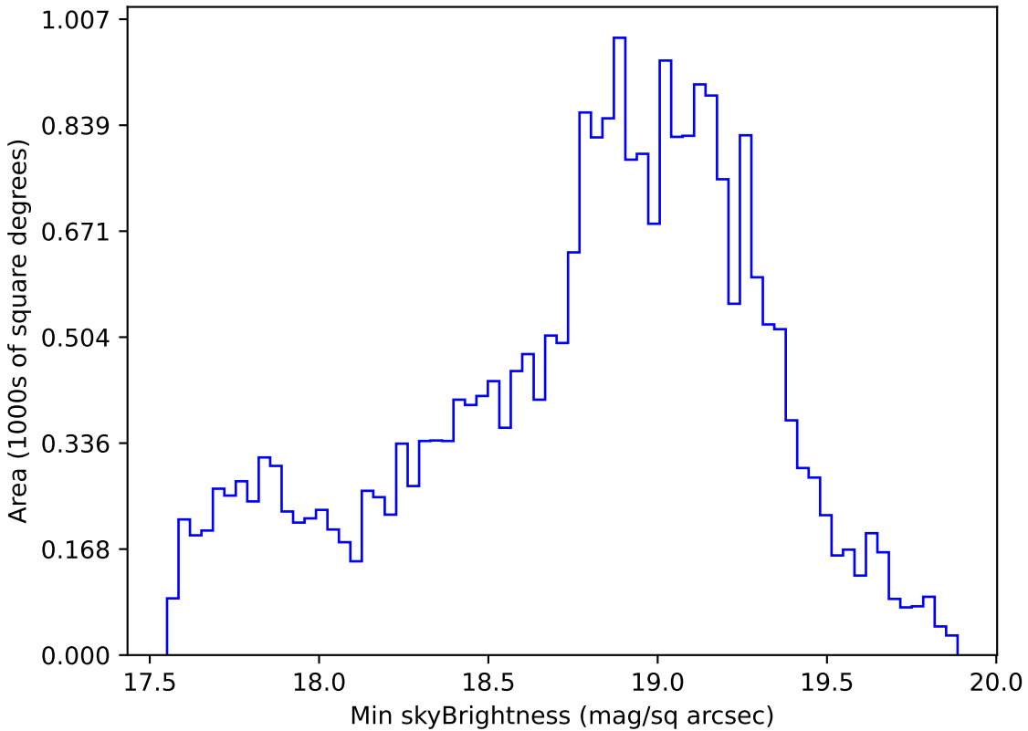
too_elab_r16_d3_ugrizy_v3.4_10yrs Yr 1 i band: Min skyBrightness
