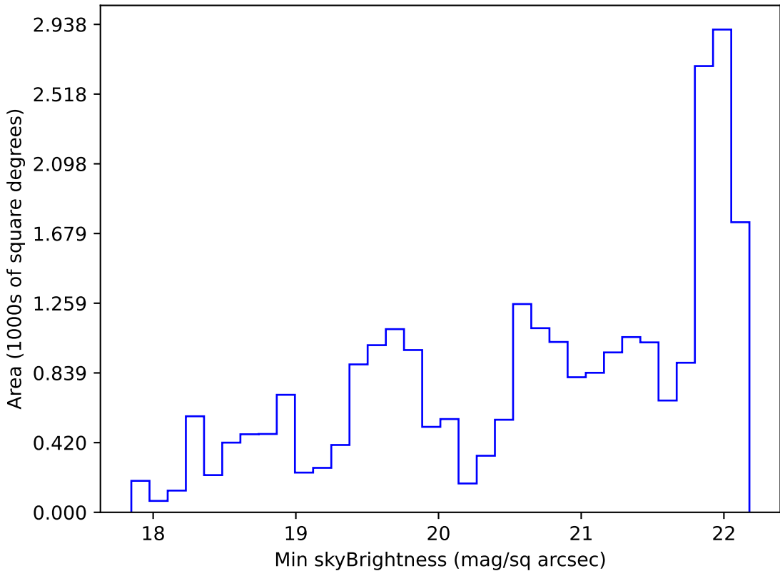
too_elab_r16_d3_ugrizy_v3.4_10yrs Yr 1 g band: Min skyBrightness
