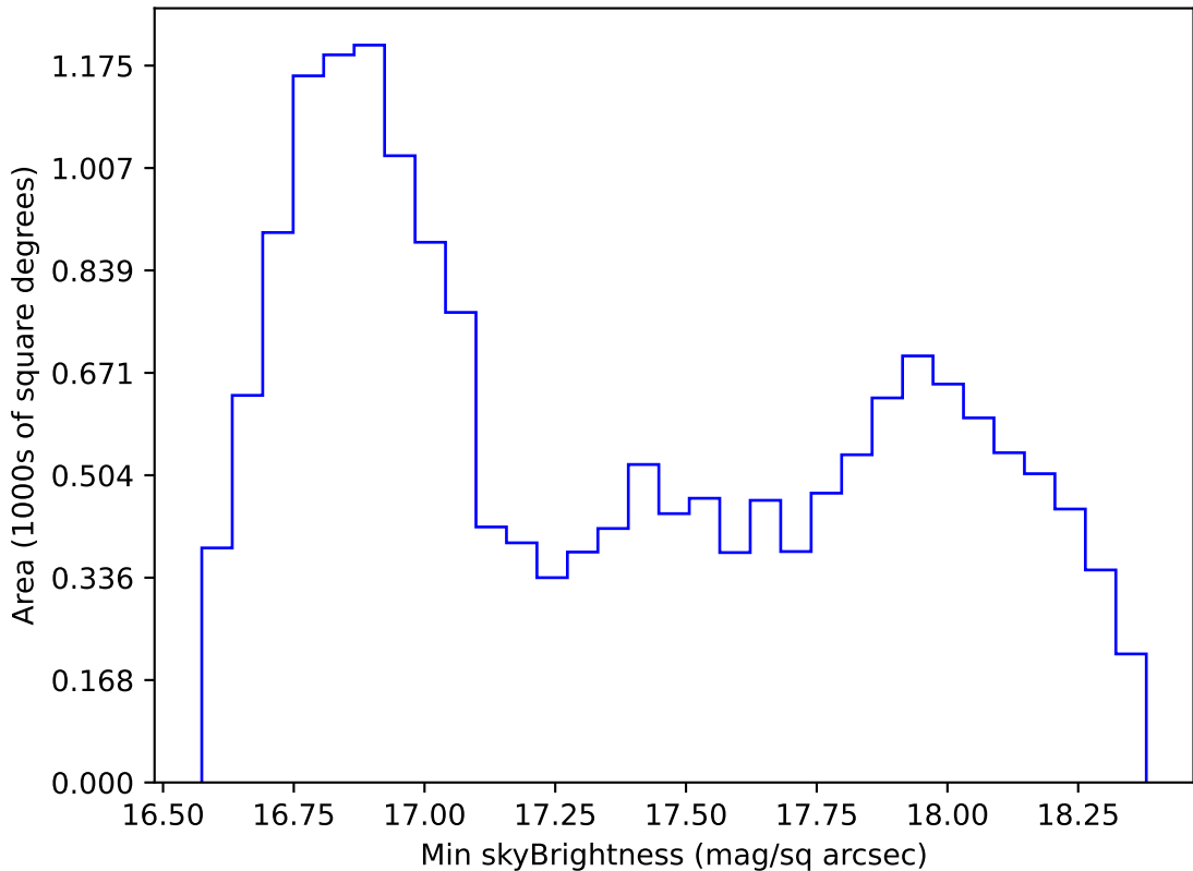
too_elab_r16_d3_ugrizy_v3.4_10yrs WFD z band: Min skyBrightness
