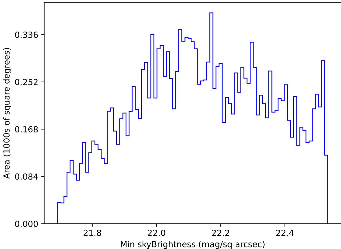
too_elab_r16_d3_ugrizy_v3.4_10yrs WFD u band: Min skyBrightness
