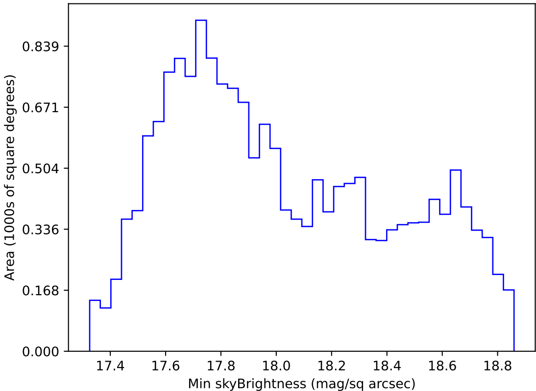
too_elab_r16_d3_ugrizy_v3.4_10yrs WFD i band: Min skyBrightness
