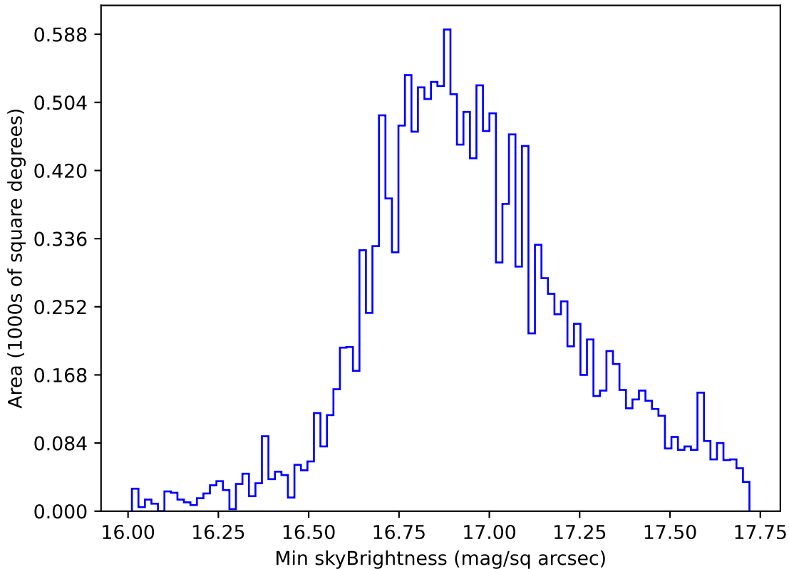
too_elab_r16_d3_ugrizy_v3.4_10yrs WFD all bands: Min skyBrightness
