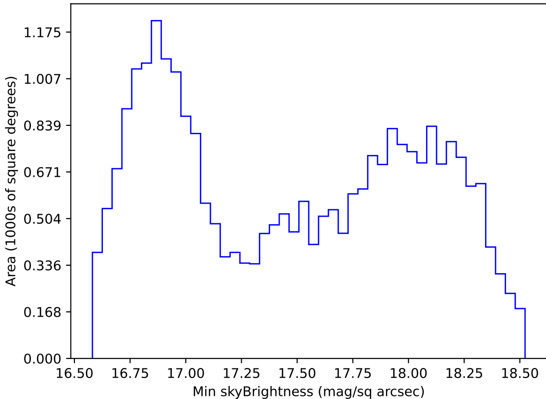
too_elab_r16_d3_ugrizy_v3.4_10yrs All sky z band: Min skyBrightness
