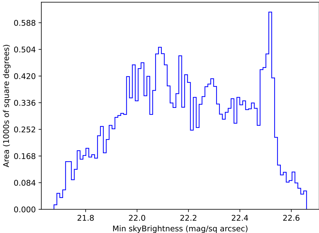
too_elab_r16_d3_ugrizy_v3.4_10yrs All sky u band: Min skyBrightness
