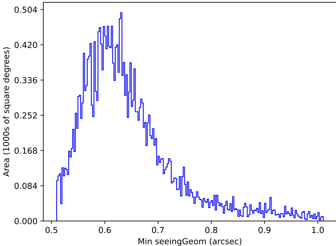
too_elab_r16_d3_ugrizy_v3.4_10yrs Yr 1 z band: Min seeingGeom
