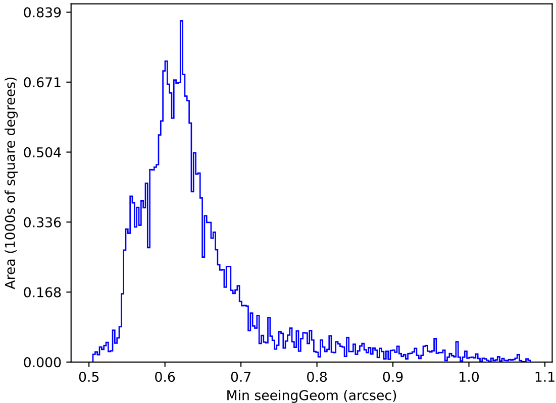
too_elab_r16_d3_ugrizy_v3.4_10yrs Yr 1 r band: Min seeingGeom
