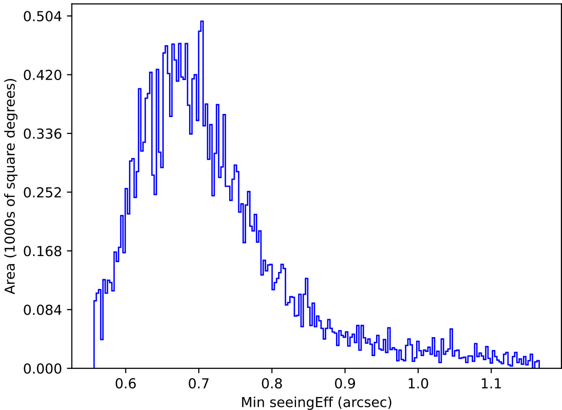
too_elab_r16_d3_ugrizy_v3.4_10yrs Yr 1 z band: Min seeingEff
